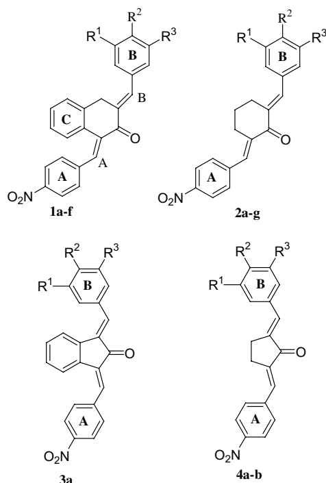
Figure 1. The general structures of compounds in series 1–4. The nature of the aryl substituents are indicated in Table 1.
